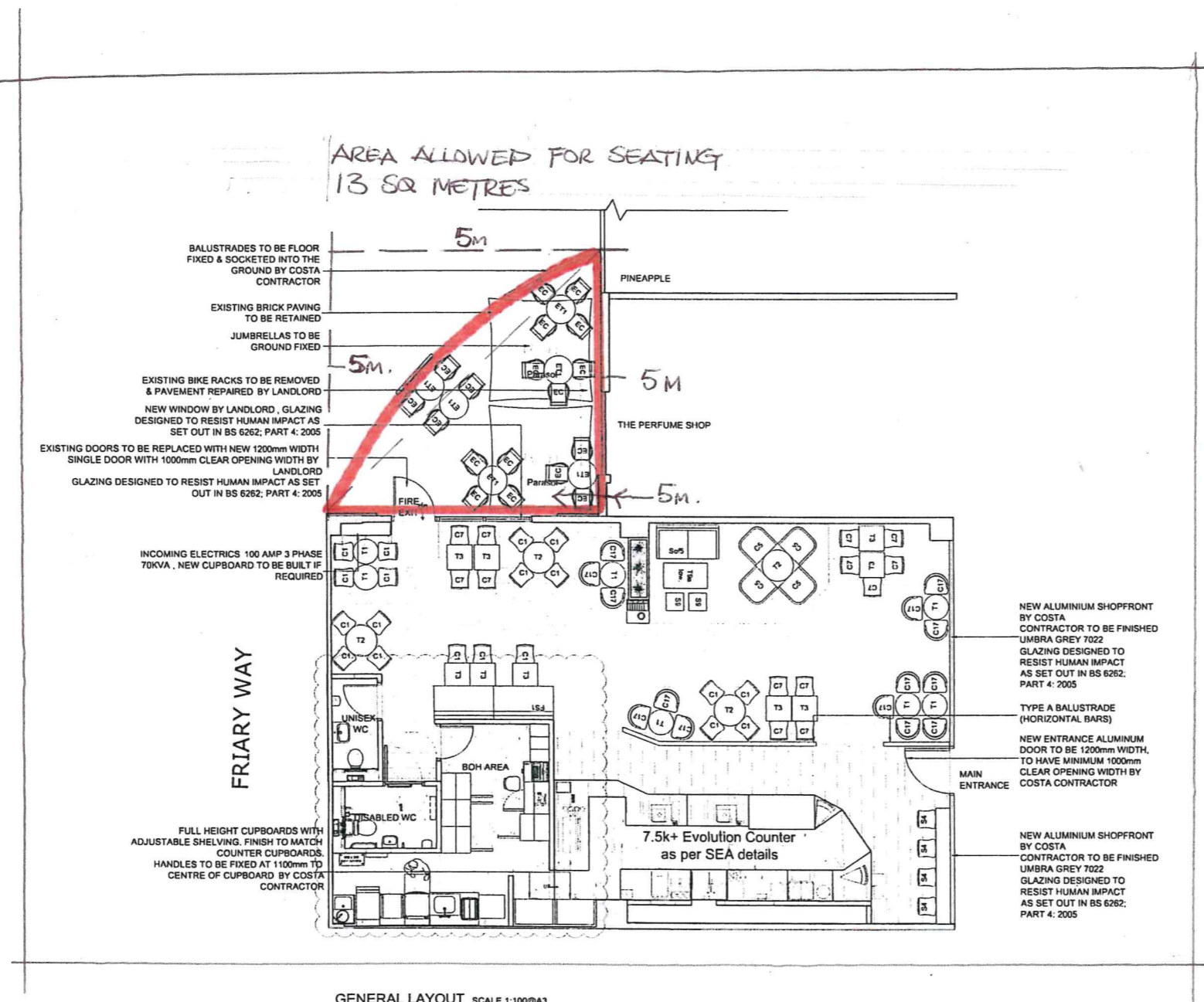
GENERAL LAYOUT SCALE 1:100@A3
